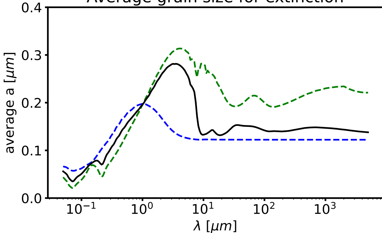
Average grain size for extinction
