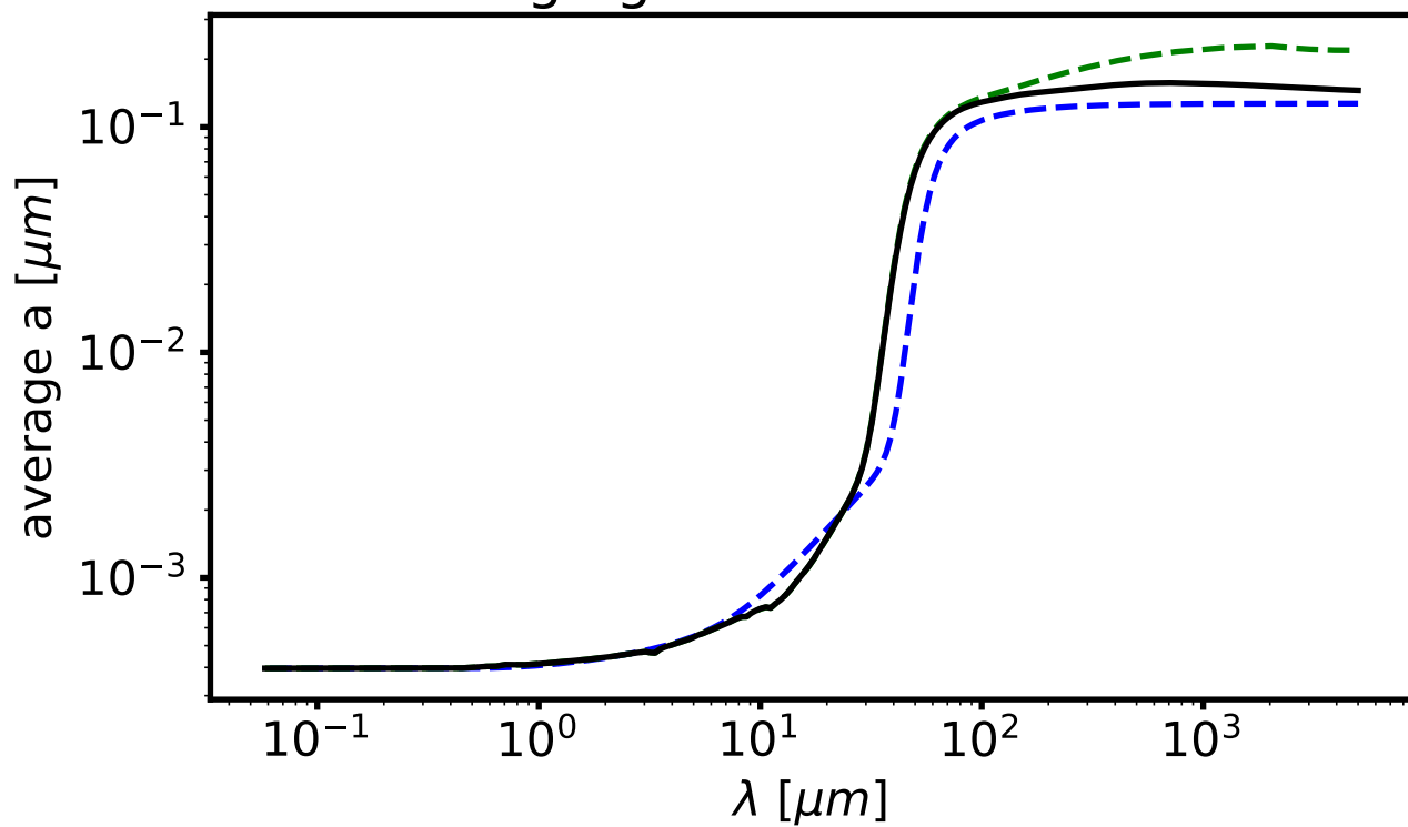
Average grain size for emission
